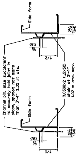
SUPPORTING CHAIR ALTERNATE
